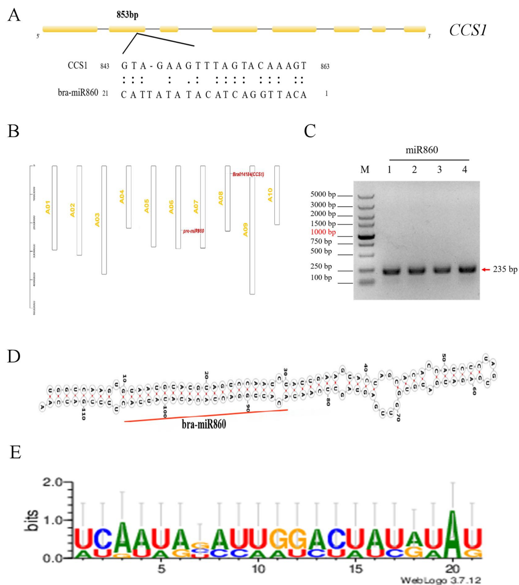
Fig S3. Information related to miR860 and its target genes. (A) miR860 target gene structure analysis and target location prediction. (B) Chromosomal localization of pre-miR860 and its target genes; (C) Lanes 1, 2, 3, and 4: miR860 precursor sequence line fragments obtained from the background genes of the maintenance line (Y231-330) and the sterility line (Tyms), respectively; (D) prediction of the secondary structure of the miR860 precursor; (E) analysis of the base conservation of the miR860 mature sequences;
