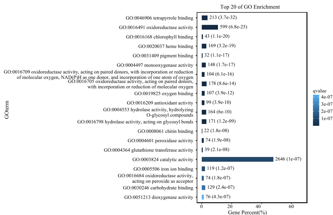
Supplementary Fig. S2: Molecular function (MF) category of GO functional enrichment analysis for differentially expressed genes (DEGs) in the CDF1_S2/CK_S1 set.
