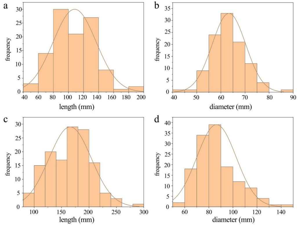
Fig. S1 Frequency distribution of fruit length and fruit diameter for F 2 -1 and F 2 -2 a, b Phenotypic distribution of eggplant fruit length and diameter in F 2 -1. c, d Phenotypic distribution of eggplant fruit length and diameter in F 2 -2.
