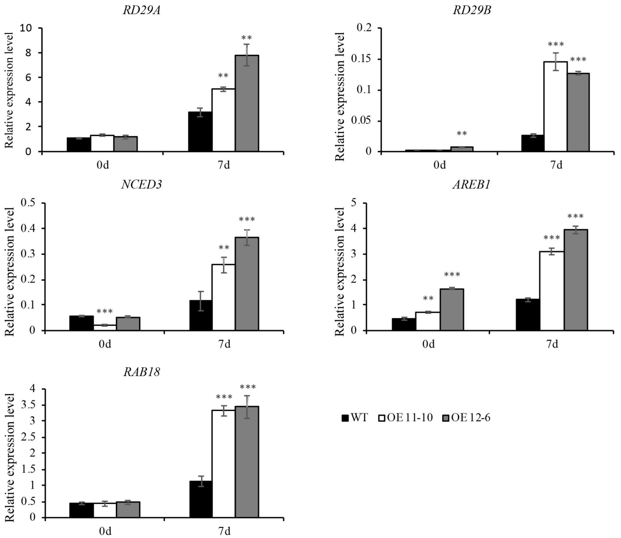
Fig. S5 The expression of drought-responsive genes in lnc000283 overexpressing lines before and after different drought treatment times. Gene expression levels were determined by RT-qPCR normalized against UBC10 ( At5g53300 ). Each value is mean \pm sd ( n = 3 ). The asterisks above the bars indicate statistical significance using Student's t -test (*, P < 0.05 ; **, P < 0.01 ; ***, P < 0.001 ).
