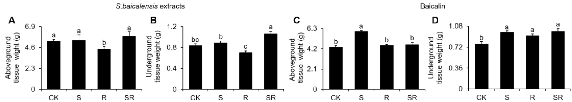
Fig. S2 Scutellaria baicalensis Georgi extracts and baicalin affect the aboveground and underground tissue fresh weight of tomato seedlings. (A, C) Fresh weight (FW) of tomato aboveground tissues after S.baicalensis extracts and baicalin treatments. (B, D) FW of tomato underground tissues after S.baicalensis extracts and baicalin treatments. Results are shown as means \pm SD (n = 6). Values marked with same letter within a sampling date are not significantly different at P < 0.05 according to Duncan's new multiple-range test.
