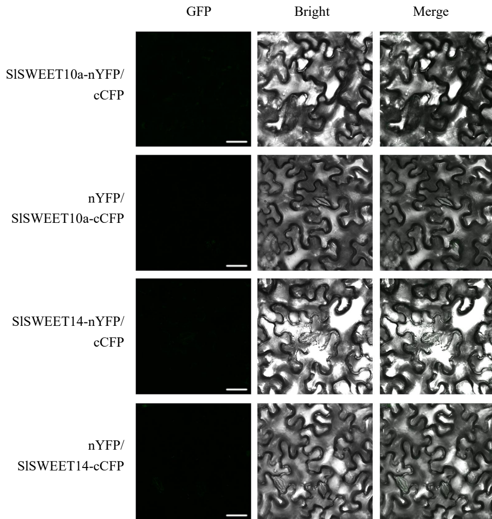
Supplementary Figure 1. Negative controls for interaction of SISWEET14 and SISWEET10a in bimolecular fluorescence complementation assays
