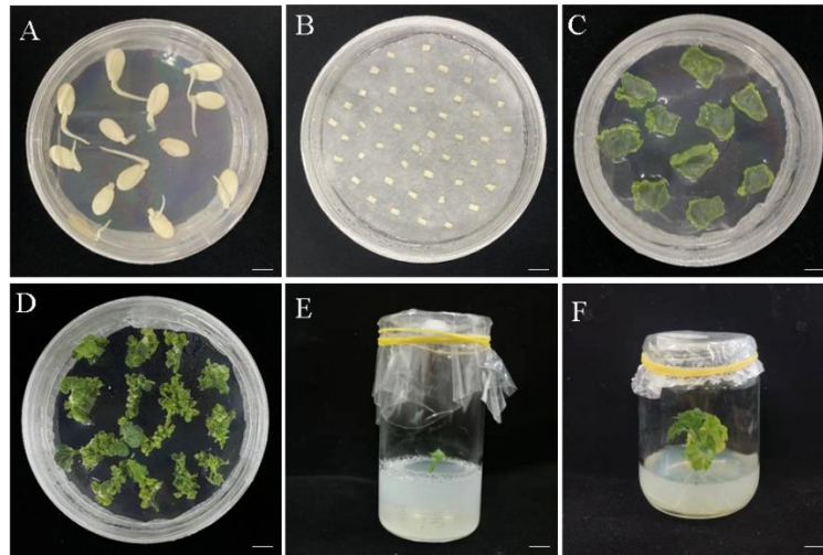
Fig. S1 Optimized stages of watermelon transformation system. (A) Seeding stage. (B) Co-cultivation stage. (C) Recovery stage. (D) Selection stage. (E) Shoot elongation stage. (F) Rooting stage. Bars=12mm.
