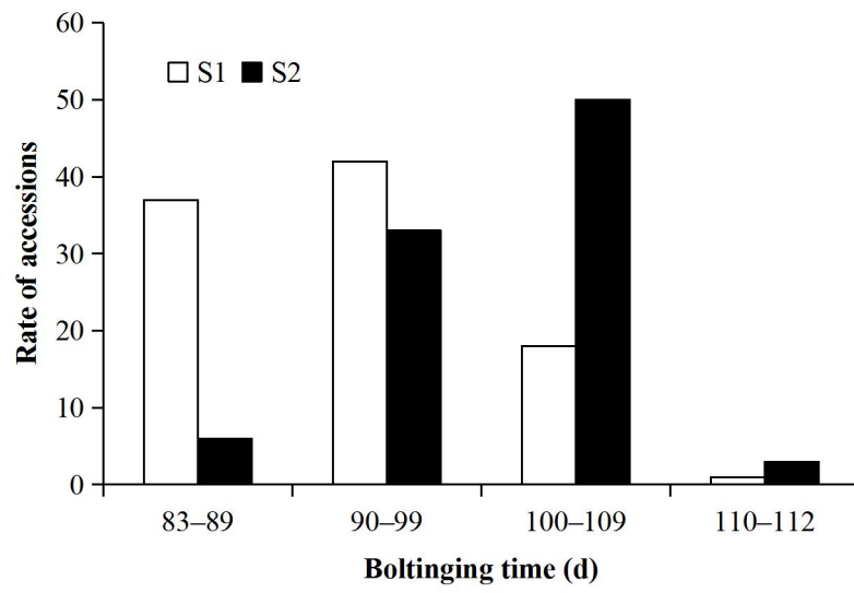
Supplementary Figure S4 Flowering time of Chinese cabbage accessions
