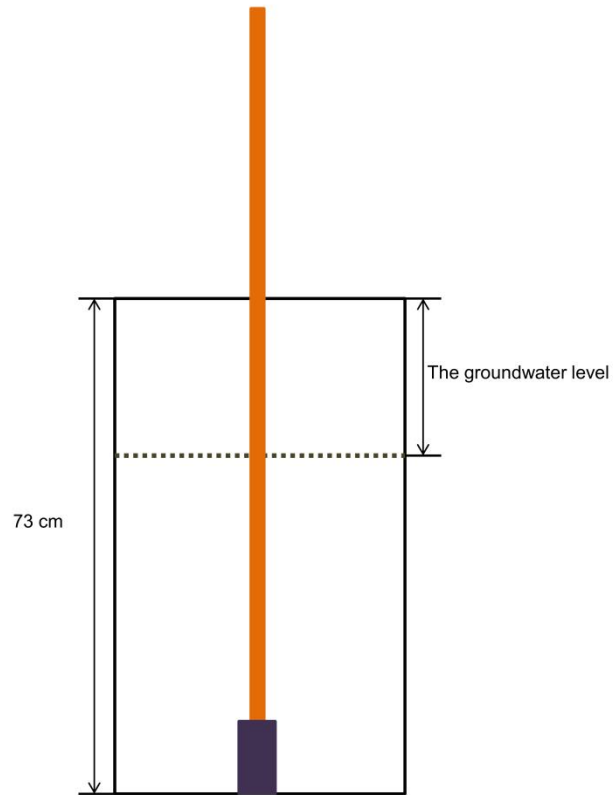
Supplemental Figure S3 The schematic diagram of water level sensor.
