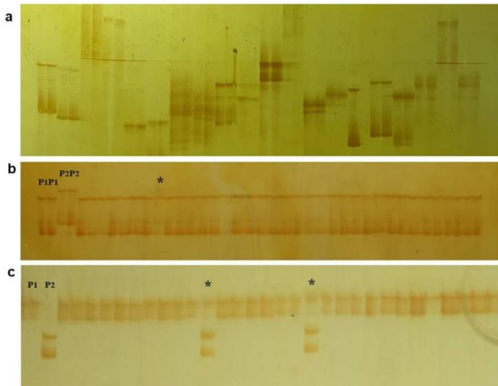
Supplementary Fig 2 Screening of molecular markers tightly linked to Brgm1 . (A) Screening of polymorphic SSR markers between the two parents. (B) Recombinants with ZMD-44 in the mapping population. (C) Recombinants with ZMD-9 in the mapping population. P 1 : mutant grm1 . P 2 : DH line '15A110'. Asterisks indicate recombinants.
