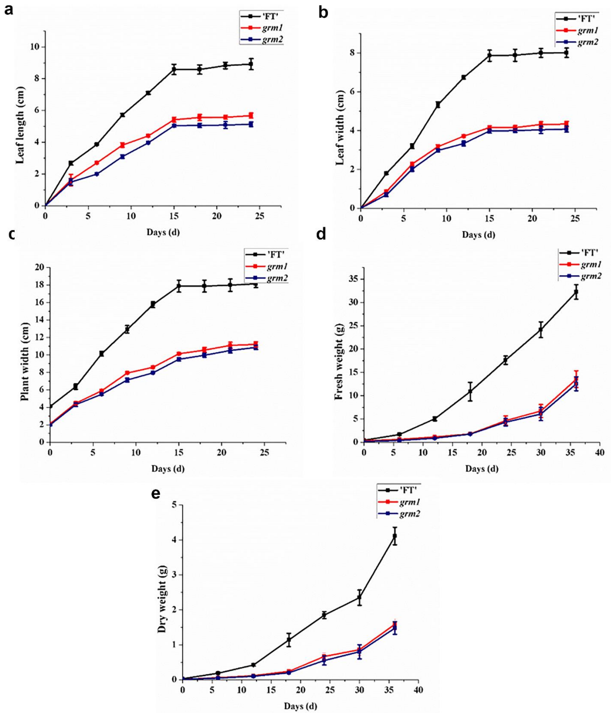
Supplementary Fig 1 Growth curve of grm1 , grm2 and 'FT' at seedling stage. (A) leaf length, (B) leaf width, (C) plant width, (D) fresh weight, (E) dry weight.
