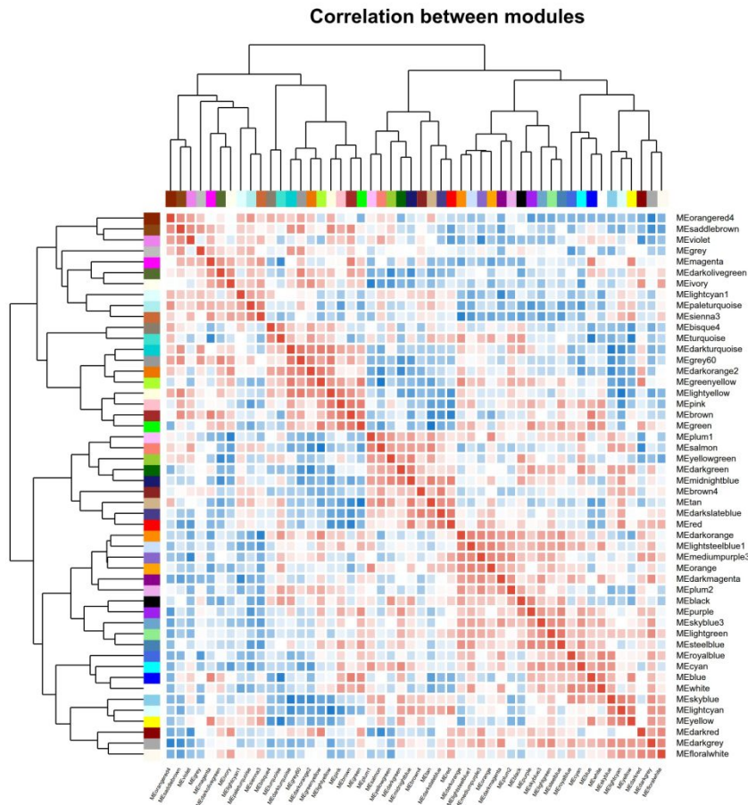
Figure S3. Heatmap and hierarchical clustering of correlations between modules. The figure illustrates the correlation levels among distinct gene modules. The rows and columns denote different module names and their corresponding colors. The color gradient from blue (0) to red (1) represents the strength of inter-module correlation, ranging from weak to strong. The dendrograms on the top and left display the hierarchical clustering of modules based on the similarity of their expression patterns; closer branches indicate higher similarity in expression patterns between modules.
