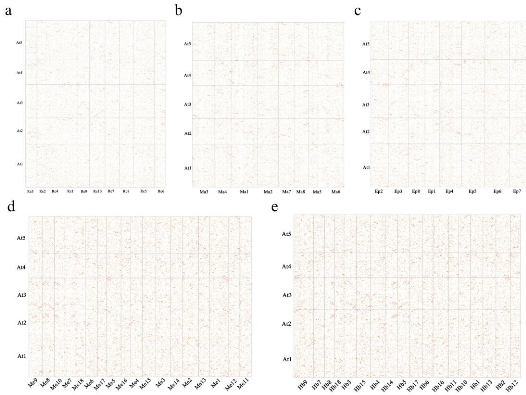
Supplementary Fig. S3 Genome dot plot within A. thaliana and 5 Euphorbiaceae species
