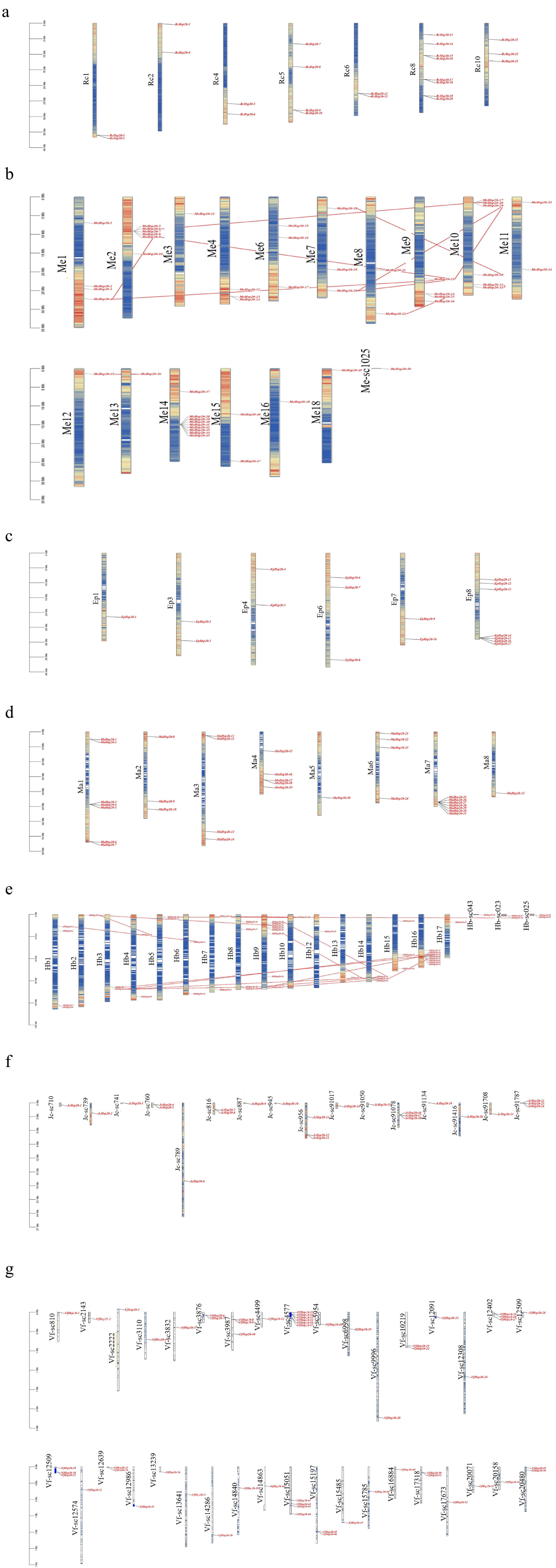
Supplementary Fig. S5 Chromosome distribution of Hsp20s from seven Euphorbiaceae species
