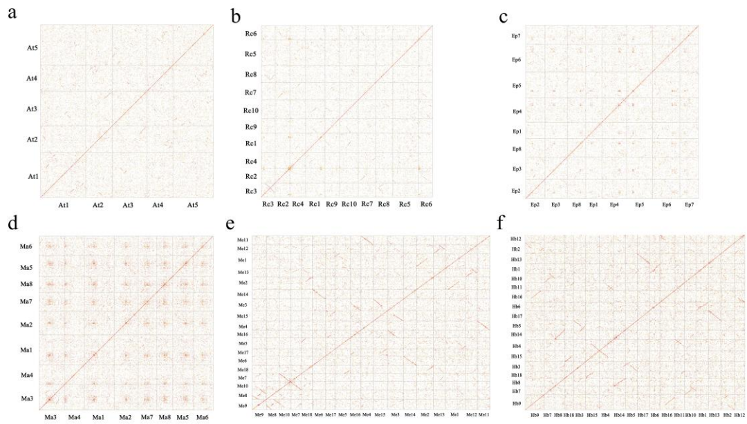
Supplementary Fig. S4 Genome-wide duplication events within species
