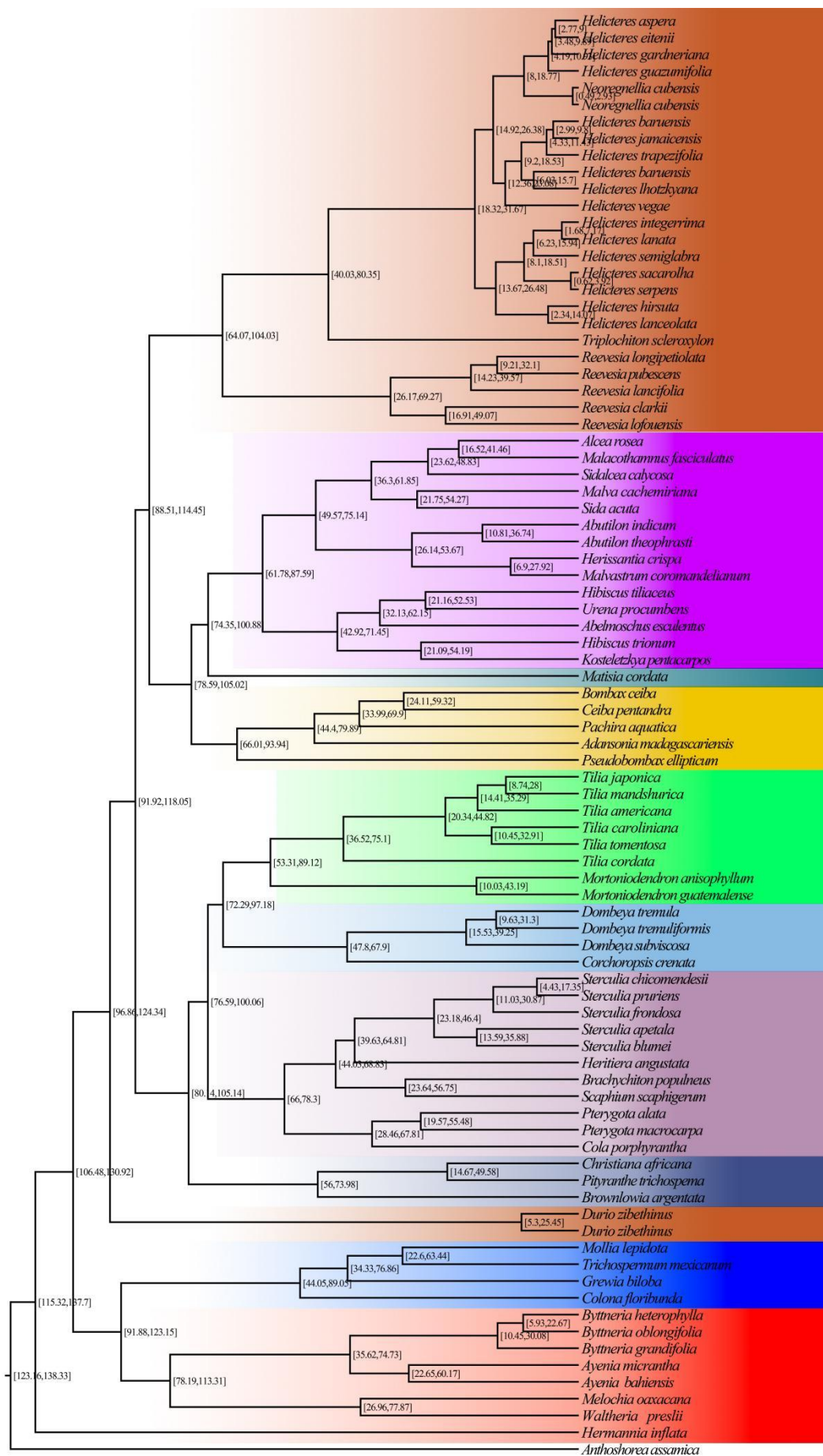
Supplementary Fig. S1 Complete time-calibrated phylogeny showing mean divergence times and their 95% highest posterior density intervals for all nodes.
