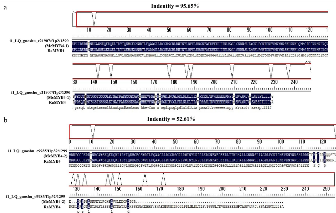
Fig. S2. Multiple alignments of RaMYB4 and two McMYBs.
