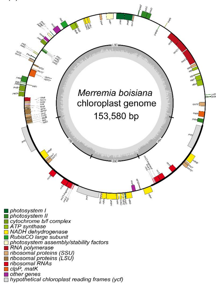
Supplementary Data Figure 2 The chloroplast genome of M. boissiana .
