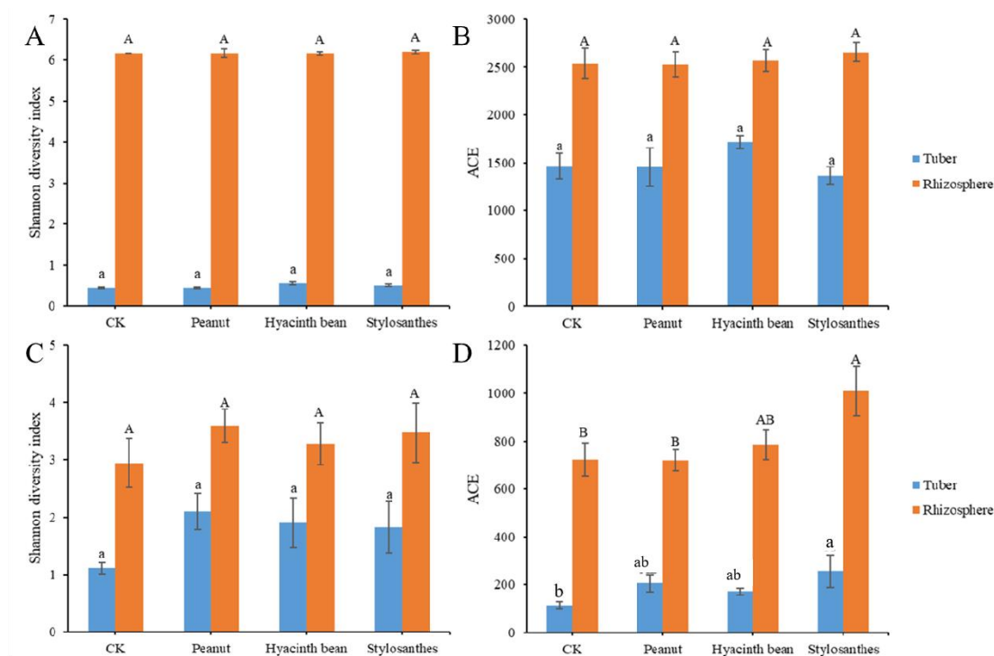
Figure S2 Tubers and rhizosphere soil microbial Shannon diversity (A. bacteria and C. fungi) and richness (abundance-based coverage estimator, ACE) (B. bacteria and D. fungi) after intercropping with different Leguminosae .
