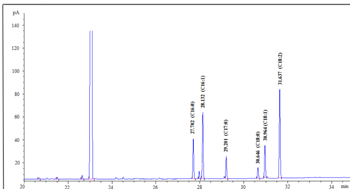
Figure S8: The fatty acid GC of S. cerevisiae with empty vector pYES2 was transformed by LA culture at 20°C.
