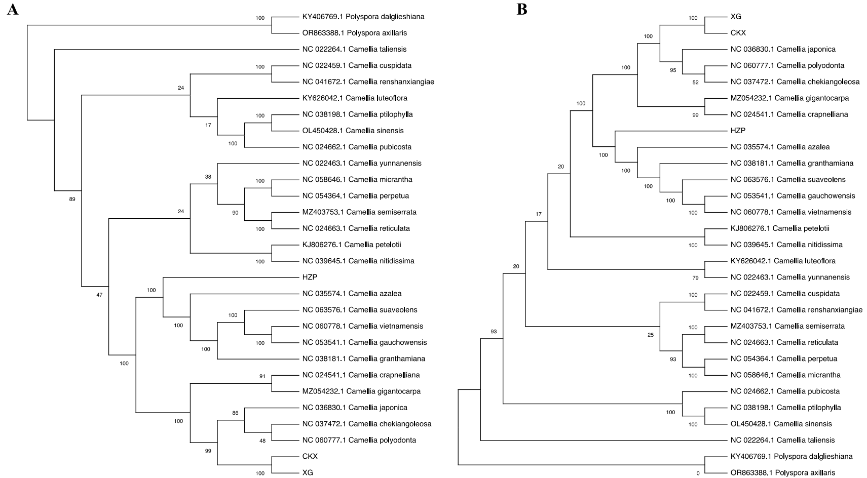
Figure S2 Phylogenetic tree reconstruction of 27 Camellia species based on whole chloroplast genome sequences by (A) ML methods and (B) MP methods.
