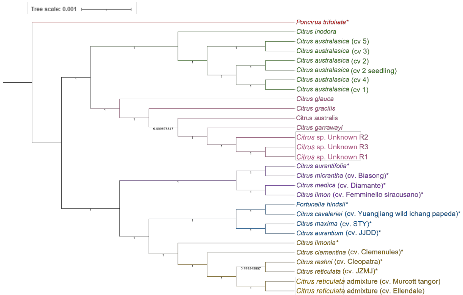
Supplementary Fig. S1 Phylogenetic tree generated from 86 nuclear genes sequences of 29 citrus samples (species/cultivars) with Poncirus trifoliata as the outgroup. The MrBayes tree was generated in Geneious. Posterior probability values are given on each node. * SRA data obtained from National Centre for Biotechnology Information for nuclear genes assembly.
