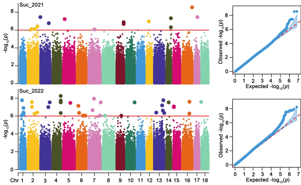
Supplementary Figure 2. Manhattan and QQ plots depict the GWAS results of Suc in 2021 and 2022. Red lines represent a p-value of 1e-6 and the dot size of significant SNPs is magnified two-fold.
