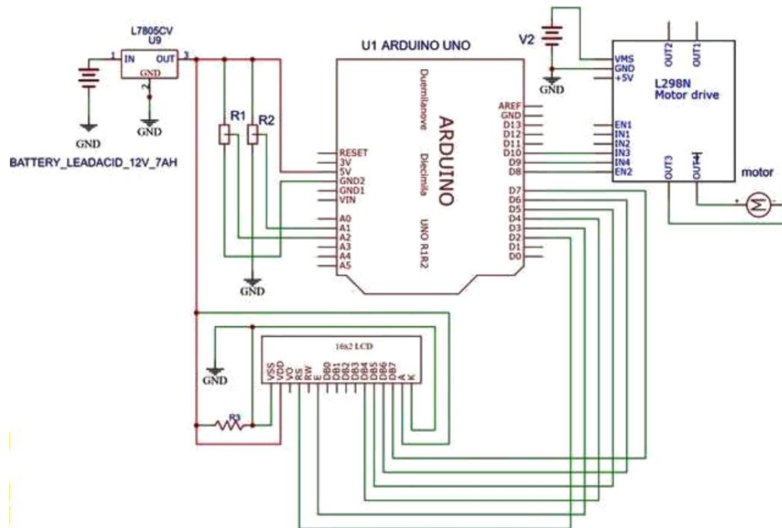
Supplementary Fig. S1 Electronic circuit of developed embedded system.
