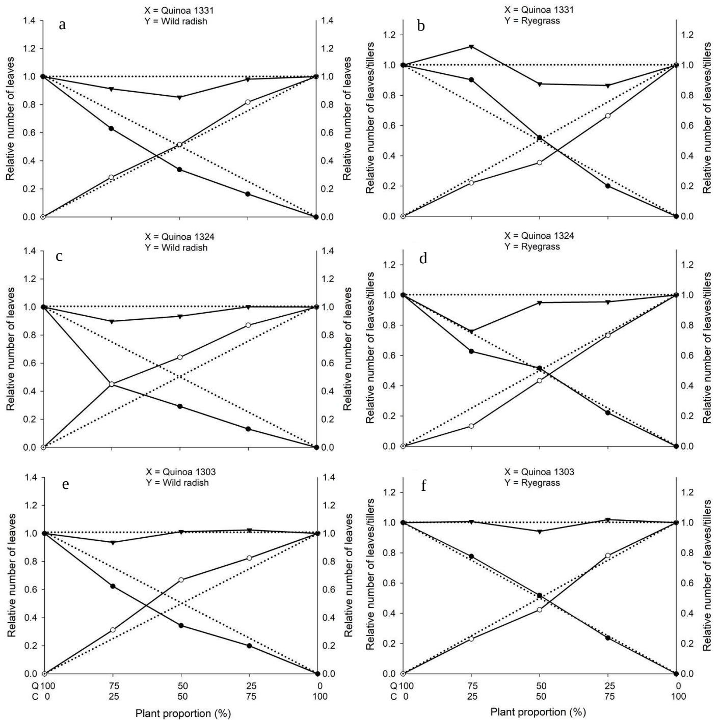
Supplementary Fig. S2 Total relative productivity (TRP), and relative productivity (RP) for leaf number of quinoa genotypes 1331, 1324, and 1303. Quinoa (●); wildradish (○: a, c and e) or ryegrass (○: b, d and f), and community (crop + weed) yields (▼). Dashed lines (---) represent the expected yields in the absence of interspecific competition, whereas solid lines (—) represent the observed values under interspecific competition. UFFS, Erechim, RS, Brazil. Q: quinoa and C: competitor.
