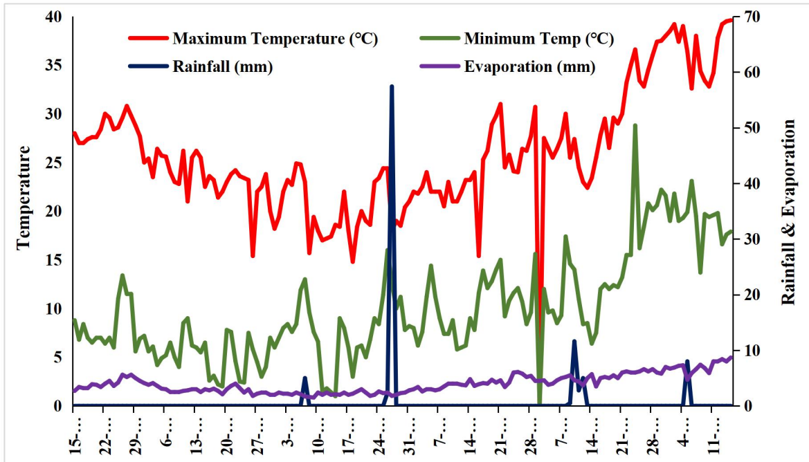
Supplemental Fig. S2 The daily weather of the experimental plot during 2016-2017
