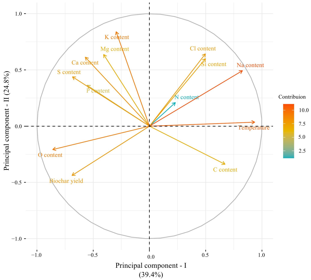
S3: PCA for the parameters influencing coconut husk biochar production; relationship between principle components -I and II
