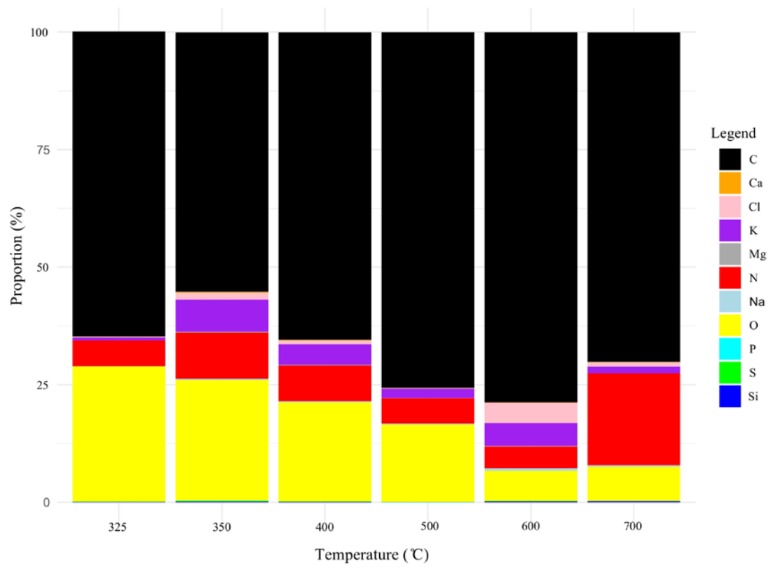
S1: Variation patterns of measured elements with the increasing pyrolysis temperature
