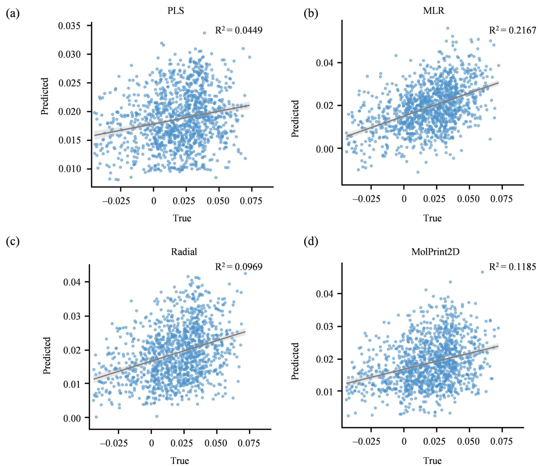
Fig. S5. Performance of DDN surpasses multiple QSAR models. a-d. Scatter plots showing the QSAR performance calculated by PLS (a) and MLR (b) in Discovery Studio, and Radial (c) and MolPrint2D (d) in Schrödinger.
