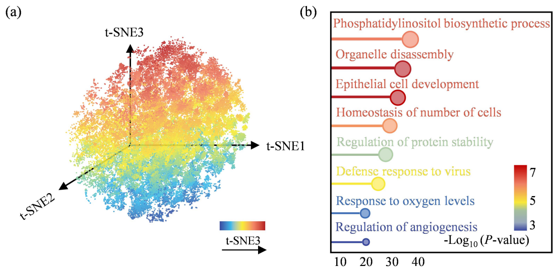
Fig. S7. LGE-GNN-Guided Identification of the NRF2 Pathway as a Key Mediator of CBD's Neuroprotective Effects. a. 3D scatter plot shows the t-SNE distribution of the training set for the linear regression model. b. Lollipop plot represents the GO enrichment pathways of the differential genes.
