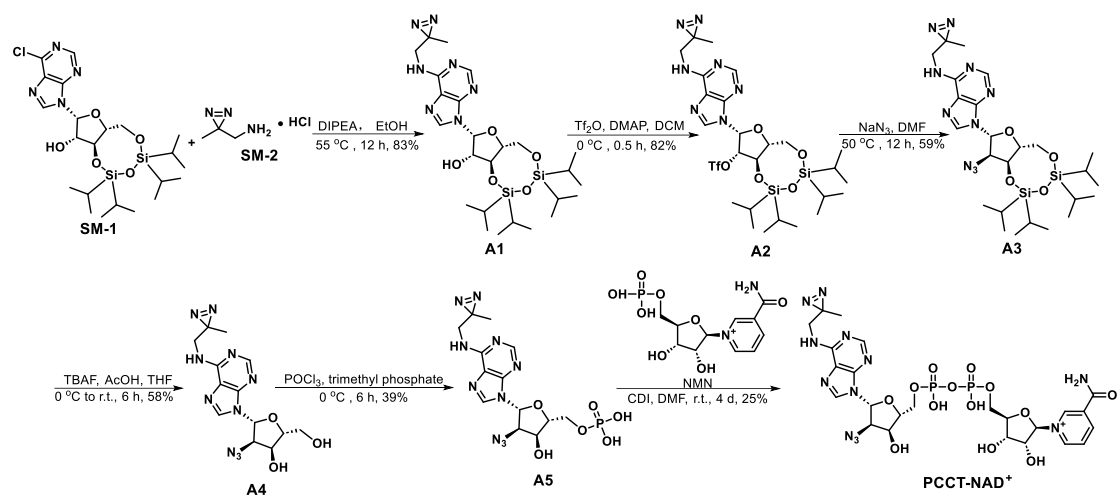
Scheme S1. Chemical synthesis of PCCT-NAD + .
