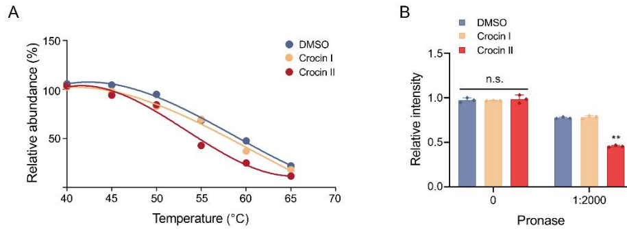
Fig. S1. Compound screenings identify Crocin II as a potential drug targeting Angptl8, referred to Fig. 1. (A) The relative protein abundance of Angptl8 in the CETSA assay. (B) The quantitative analysis of protein levels of Angptl8 in the DARTS assay. n = 3 , n.s., no significance, **P < 0.01 v.s. DMSO group, one-way ANOVA followed by Bonferroni's posthoc test. All values are presented as the mean \pm SD.
