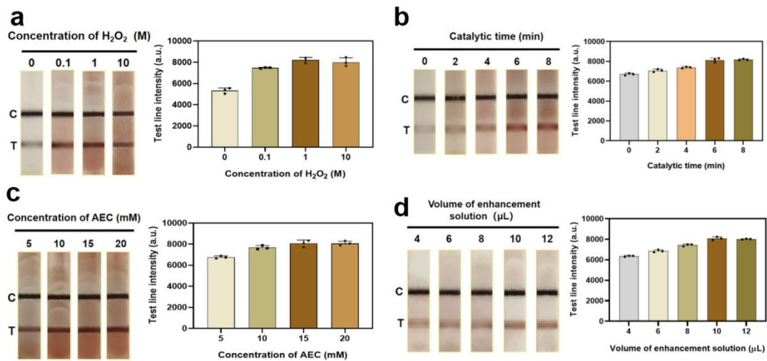
Figure S9. Optimization photographs of enhancement solution. (a) Strips and relative intensity of test line with different concentration of H 2 O 2 , (b) catalytic time, (c) concentration of AEC substrate, (d) volume of enhancement solution. Error bars denote the standard deviation (n = 3).
