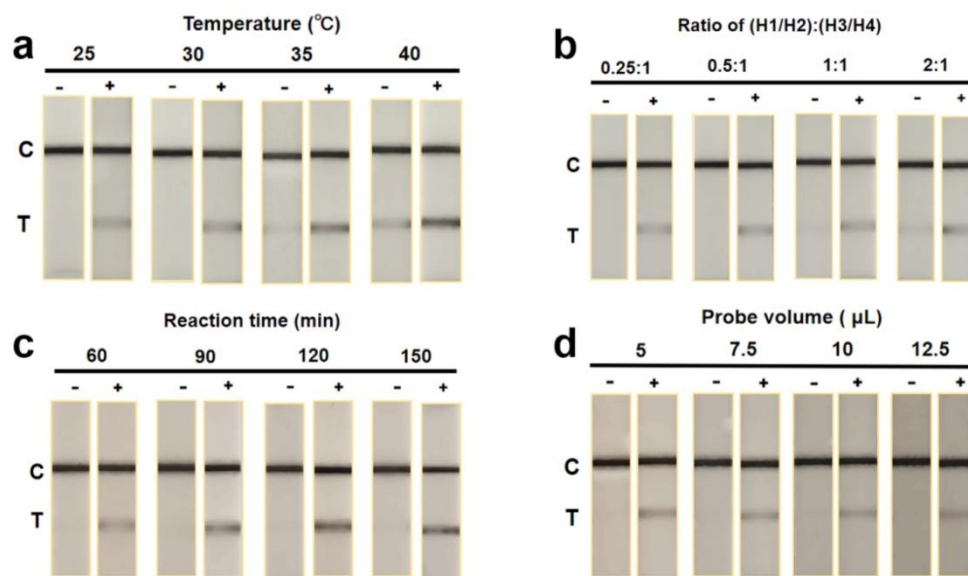
Figure S8. Optimization photographs of mbLFIA reaction conditions. (a) Relative T line intensity of positive and negative samples under different temperatures. (b) Different concentration ratios of (H1/H2) to (H3/H4). (c) Different reaction times. (d) Different volumes of Au@Pt-DNA probe.
