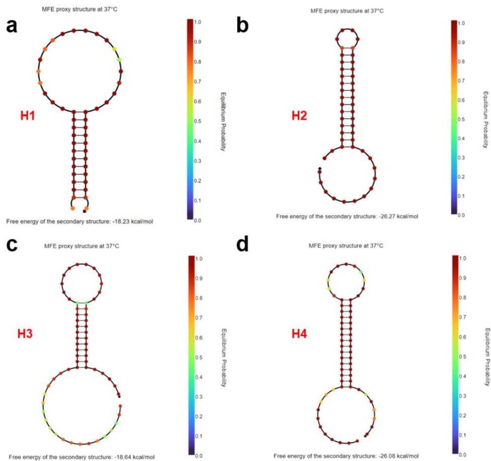
Figure S6. NUPACK-predicted secondary structures and Gibbs free energies for (a) H1, (b) H2, (c) H3, (d) H4. Parameters were set as 37 °C, Na + (100 mM), Mg 2+ (0 mM), DNA (100 nM).
