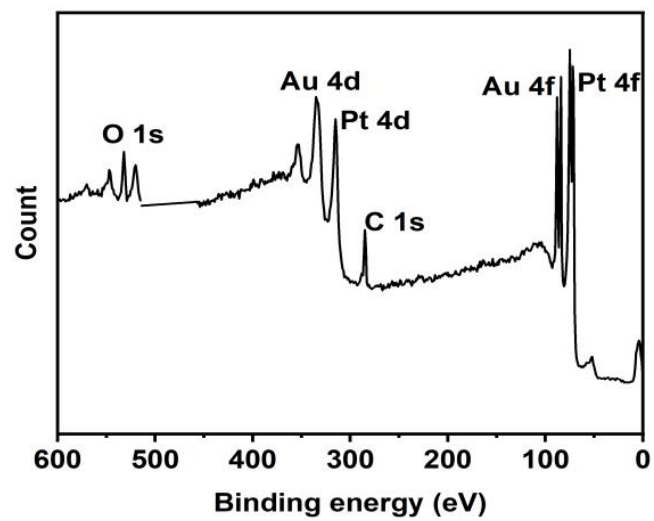
Figure S2. XPS full spectrum of Au@Pt NP
