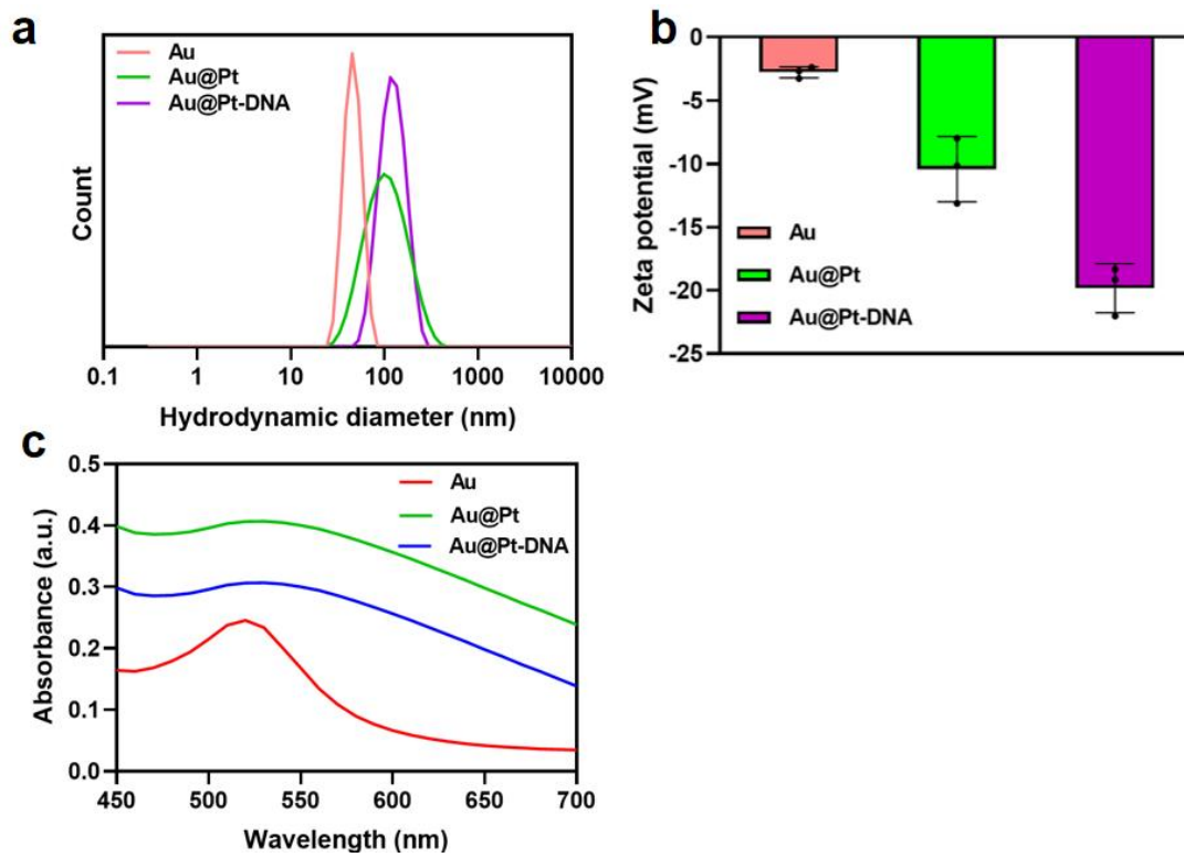
Figure S5. (a) The different change between Au, Au@Pt NP, Au@Pt-DNA of hydrodynamic diameter, (b) zeta potential and (c) UV absorbance. Error bars denote the standard deviation ( n = 3 )
