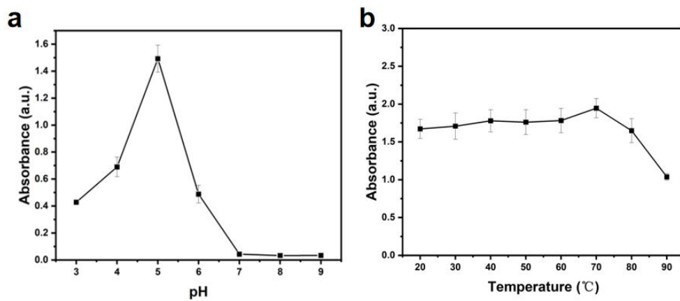
Figure S4. Stability of the catalytic activity of Au@Pt NPs. (a) The catalytic activity of Au@Pt NPs in different pH and (b) temperature condition for TMB. Error bars denote the standard deviation ( n = 3 ).
