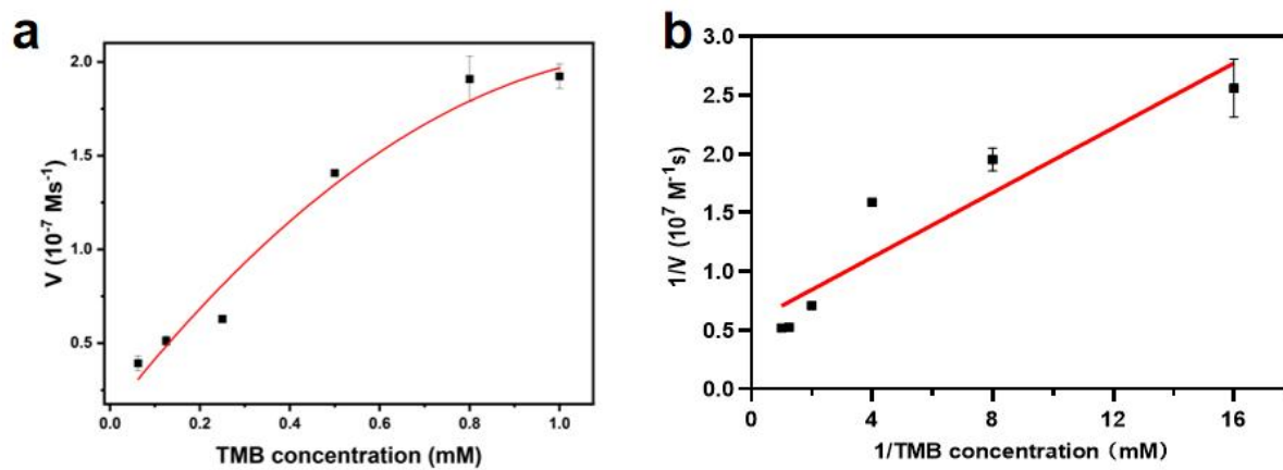
Figure S3. Steady-state kinetic assay of Au@Pt NPs based on POD-like activity. (a) TMB concentration dependence of initial reaction velocity, (b) double reciprocal plots between reaction velocity and TMB concentration. Error bars denote the standard deviation ( n = 3 ).
