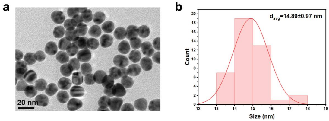
Figure S1. (a) TEM image of Au NP; scale bar is 20 nm. (b) Particle size distribution histogram of Au@Pt nanoparticles based on TEM analysis.
