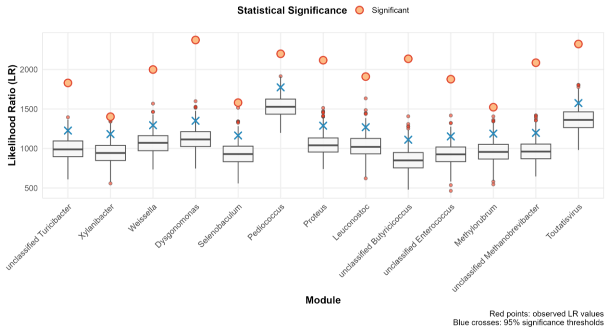
Figure S3. Statistical Significance Testing of M4 Microbial Likelihood Ratios via Permutation Test.
