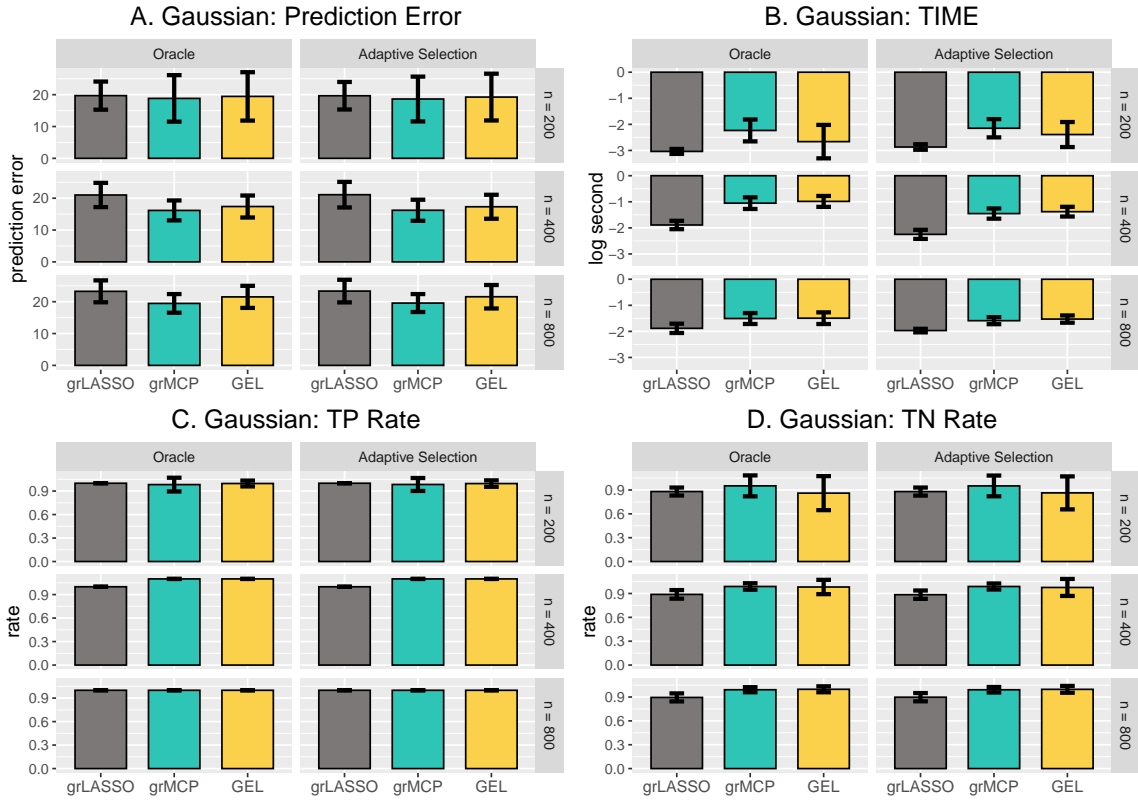
Figure S2: Results of the linear model with respect to Scenario 2. Each panel represents a different evaluation metric: prediction error (A), computing time (B), true positive rate (C), and true negative rate (D). The height of each bar indicates the average value of the corresponding metric across multiple simulations, with error bars representing twice the standard deviation. The first three bars in each panel correspond to the oracle number of factors per group, while the last three bars represent the adaptively selected numbers of factors.
