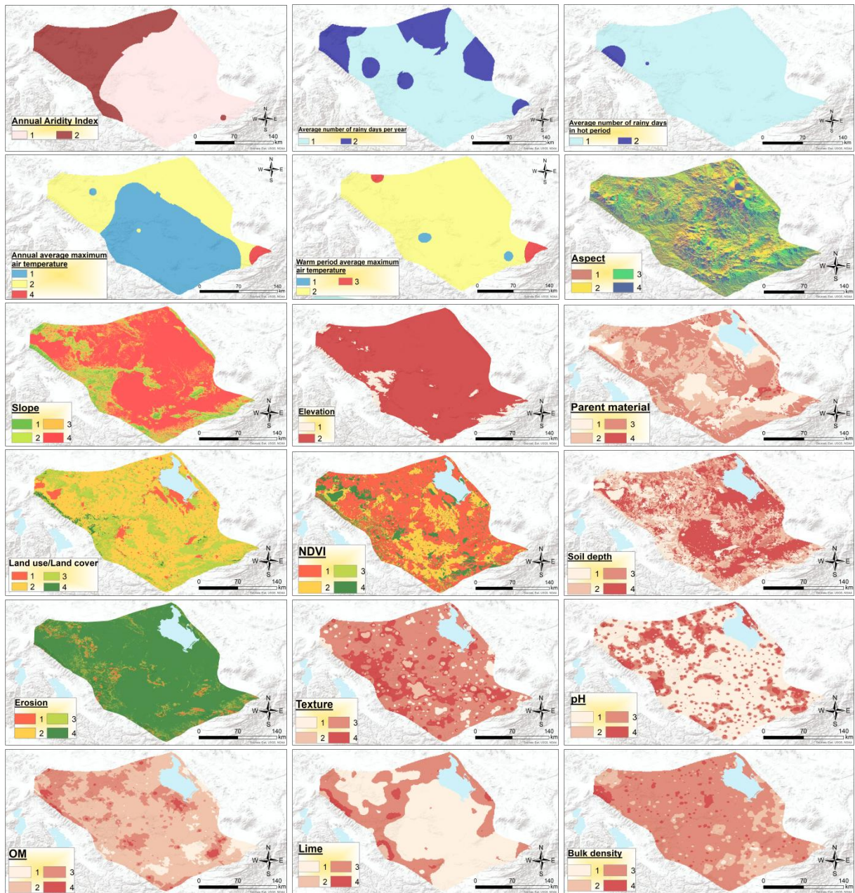
Supplementary Fig. S1. Distribution maps of criteria's index class in Konya sub-region.
