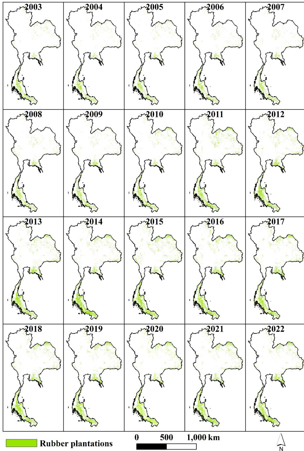
Figure S2. Spatial distribution of rubber plantations during 2003–2022
