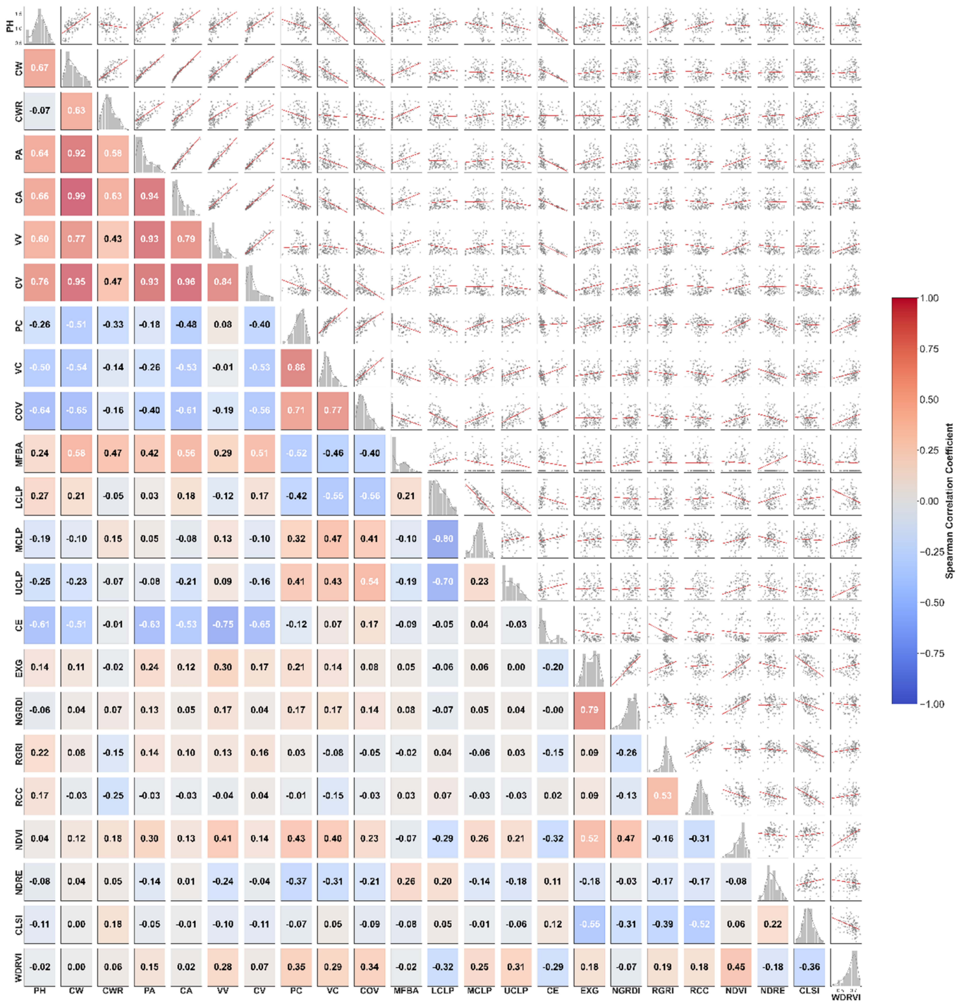
Fig.S1. Spearman Correlation Linear Matrix Plot
