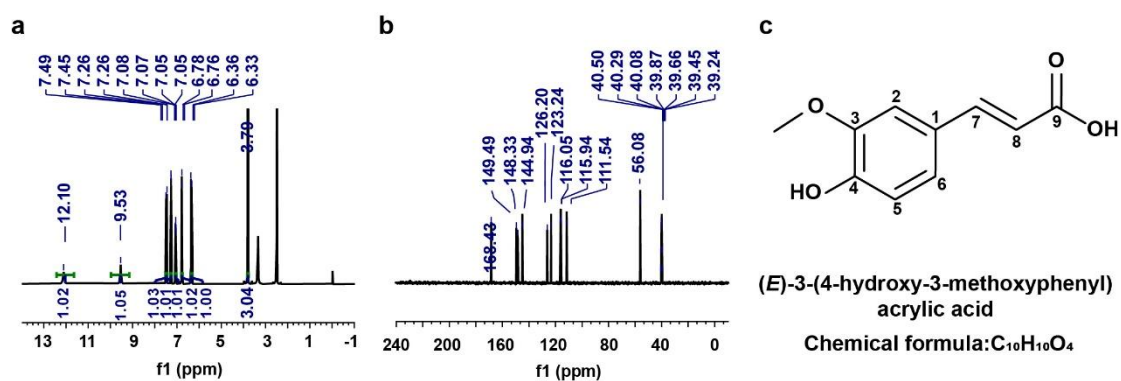
Figure S1. The MR spectroscopy and structure of Peak 1 are consistent with ferulic acid. The hydrogen spectrum (A) and carbon spectrum (B) of Peak 1. C. the structure of the compound in Peak 1 as ferulic acid.
