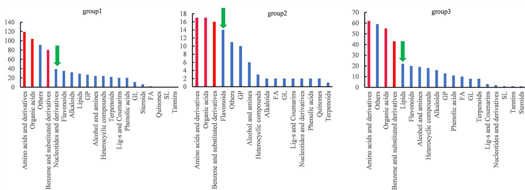
Supplementary Figure 3. Categorization of DAMs. The DAMs were classified into three main groups. The top 3 metabolites except unknown metabolites in each group were showed with red bar, and the 4th rank metabolites was indicated by green arrows.
