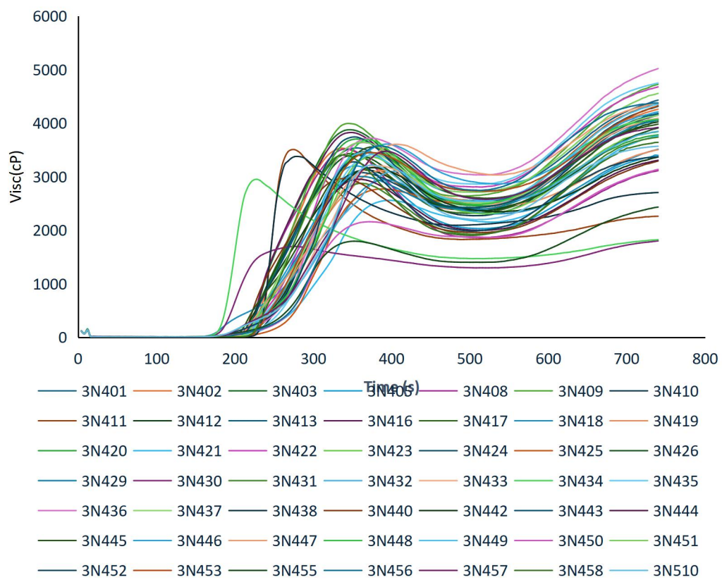
Supplemental Figure S2: Rapid Visco Analyzer (RVA) Profiles of Malaysian Rice Varieties planted in China.
