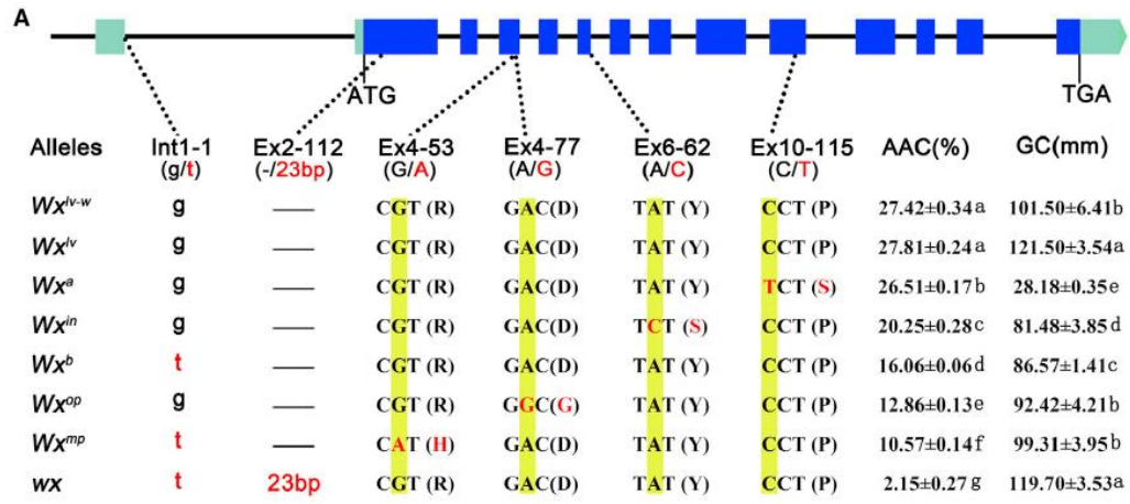
Supplemental Figure S1: Genotypes and phenotypes of different Wx alleles. The top section illustrates the genomic structure of the Wx gene, and the nucleotide sequences and their corresponding amino acid residues (shown in parentheses) at six key functional polymorphic sites are listed for each allele. On the right, the amylose content (AAC) and gel consistency (GC) of mature grains from near-isogenic lines (NILs) carrying the respective Wx alleles are displayed (Zhang et al. 2019).
