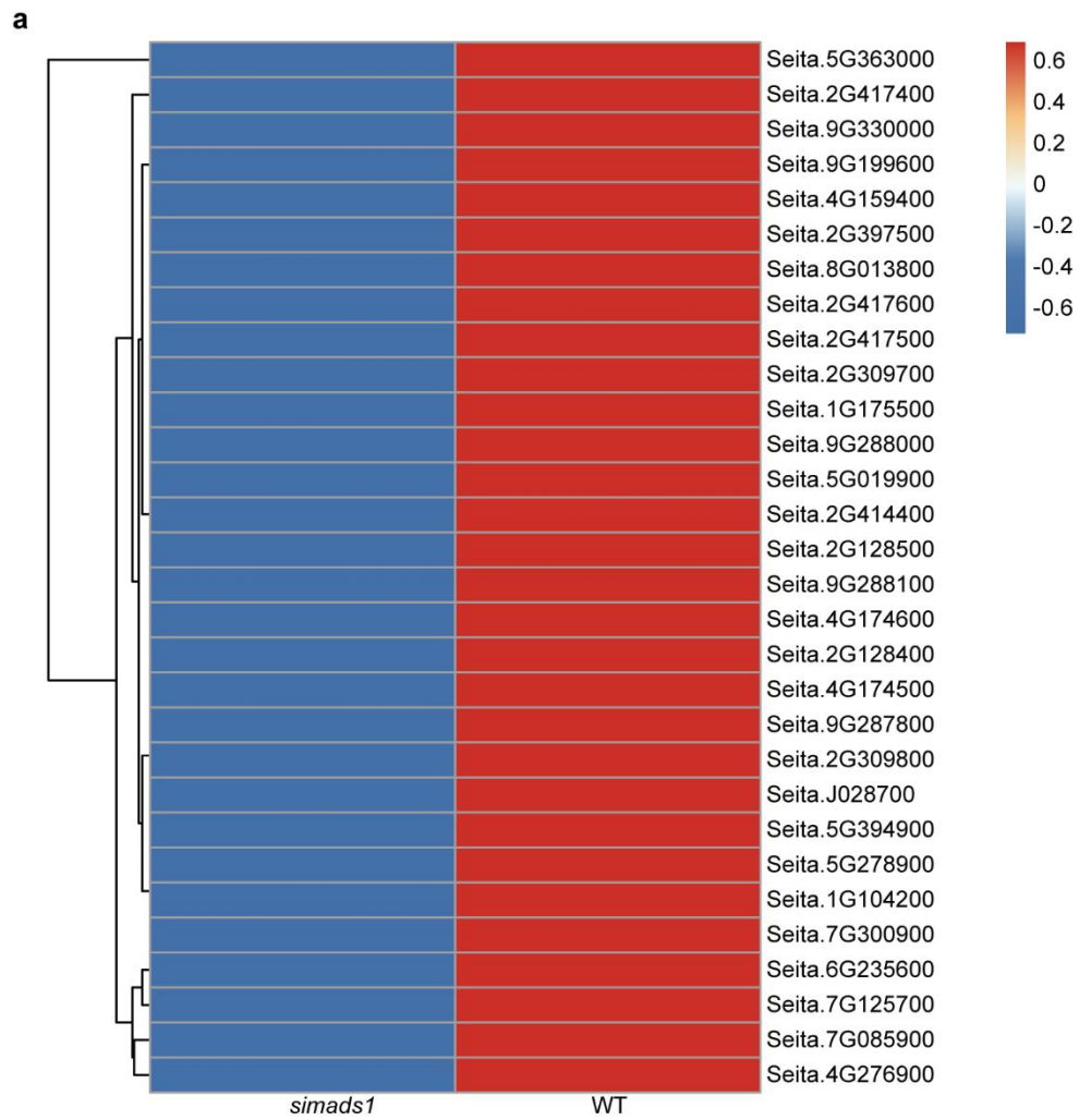
Supplemental Fig 8. Expression feature of the non-specific lipid transfer proteins (LTP) simads1 and WT in panicle period.
